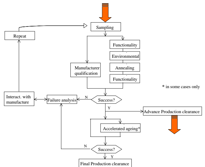
Figure 4: Flow chart of the pre-production qualification procedure.
