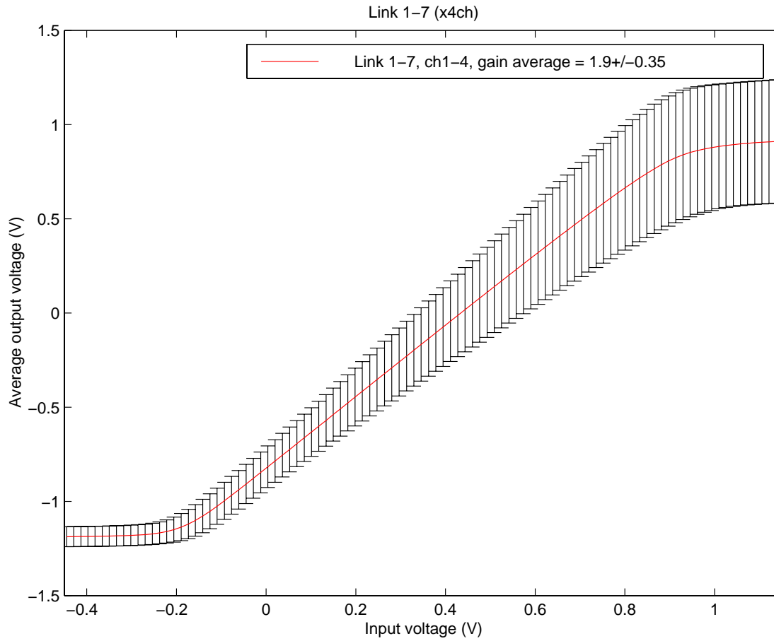
Fig 5: Average and standard deviation of link transfer characteristics over 28 channels (measured into 50\Omega ).
