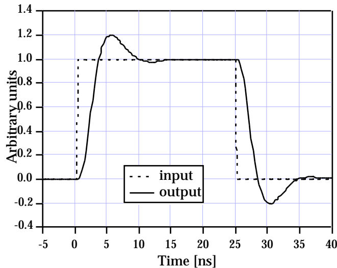
Fig. 14 : Temporal step response calculated from the inverse Fourier transformation of the link frequency spectrum (approximated as a 2nd order minimal phase network).
