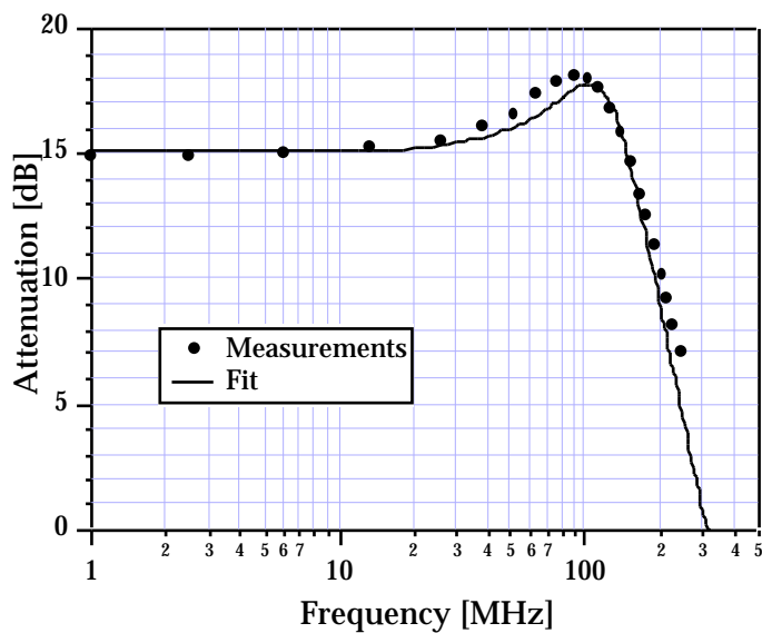
Fig. 13 : Full link frequency response. Dots are the experimental data and the line is a fit using a second order filter.
