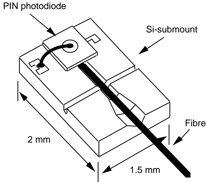
Fig. 8: Photodiode assembly showing the Si-submount, photodiode, and optical fibre.
