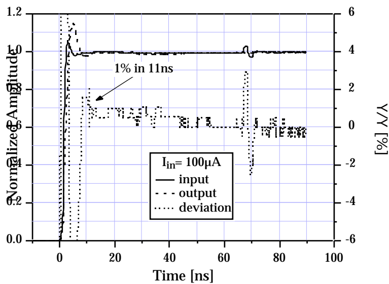
Fig. 10 : Receiver settling time to a step input signal.
