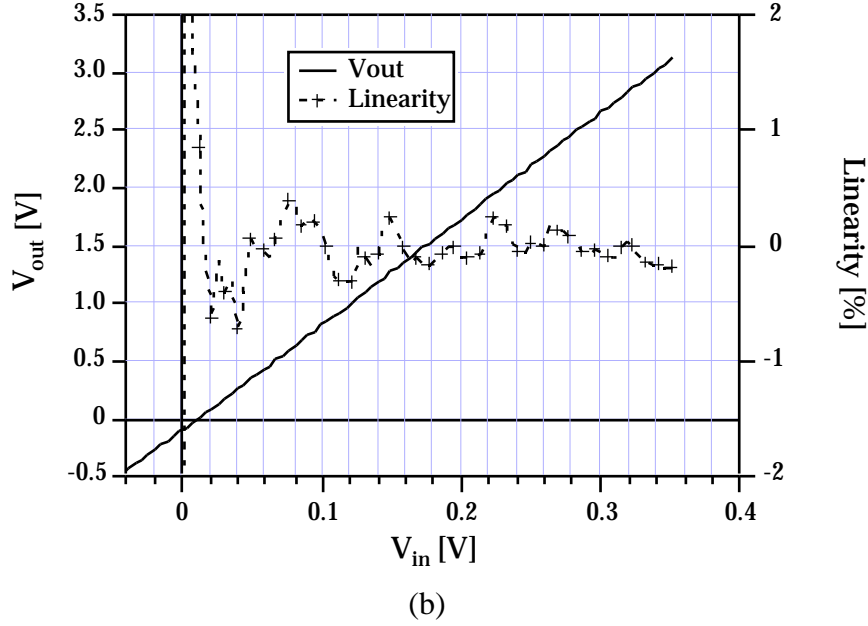
Fig. 11 : (a) Full link transfer characteristic. (b) Linearity over the 0-3V operating range of the ADC.
