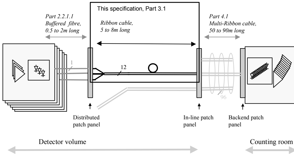
Figure 2.1, Ruggedized Ribbon highlighted in the optical link cabling structure.
