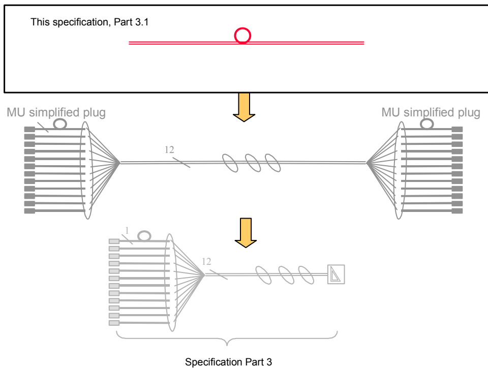
Fig. 2.2. Ruggedized Ribbon and associated components block diagram
